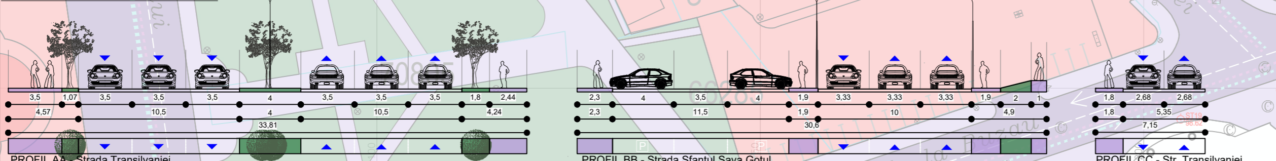
PROFILE STRADALE, scara 1 : 250
